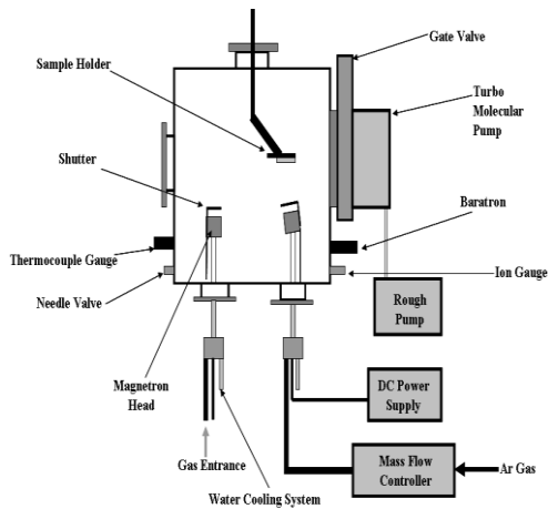
Fig. 2. The schematic of the high vacuum magnetron sputtering system.
