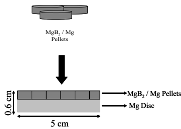
Fig. 1. Fabrication schematic of the MgB_2/Mg composite target.
