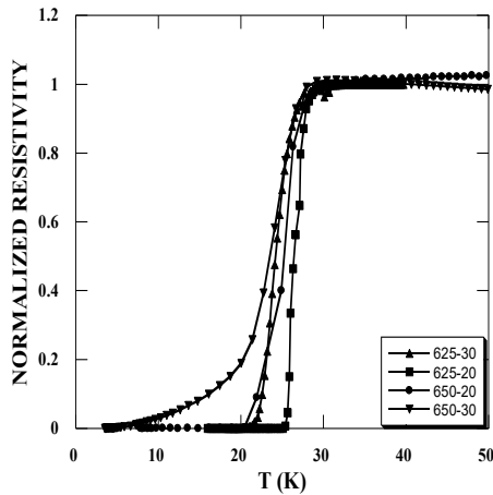
Fig. 4. R-T results for annealed films.
