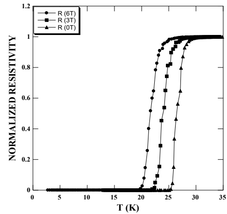
Fig. 5. R-T results for 625 °C-20 min annealed films under various magnetic fields.
