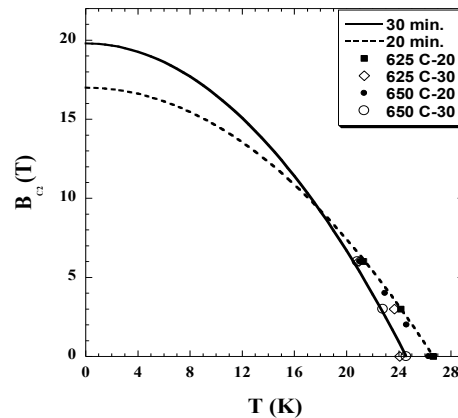
Fig. 6. Upper critical magnetic field versus temperature.
