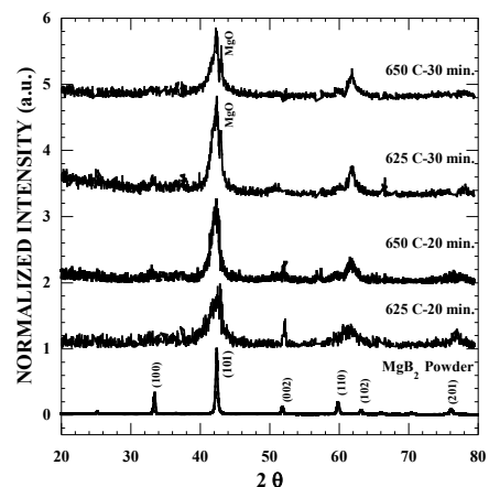
Fig. 3. XRD results for annealed films and MgB_2 powder.
